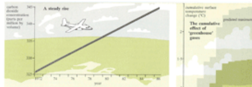
Samples of air collected by aircraft flying high over south-eastern Australia show a steady rise in the amount of carbon dioxide in the atmosphere.
